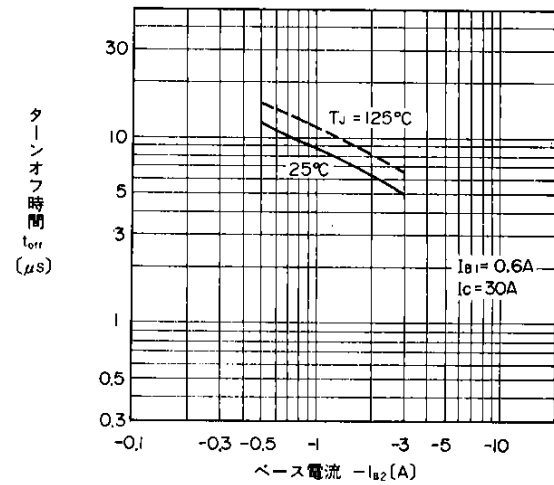
I_{B2} 依存性特性 I_{B2} Dependence of Turn off Time
