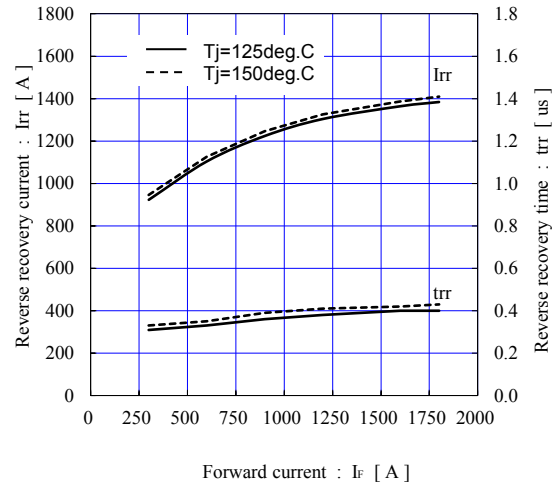
Reverse recovery characteristics (typ.) Vce=900V, VGE=±15V, Rgon=1.2Ω
