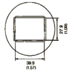
A1264 QFP 40 × 40 (1.57 × 1.57)
