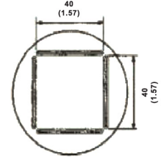
A1263 QFP 28 × 40 (1.1 × 1.57)
