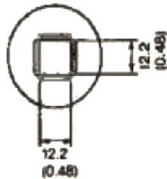
A1262 QFP 12 × 12 (0.47 × 0.47)
