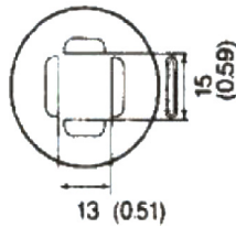
A1140 PLCC 11.5 × 11.5 (0.45 × 0.45)
