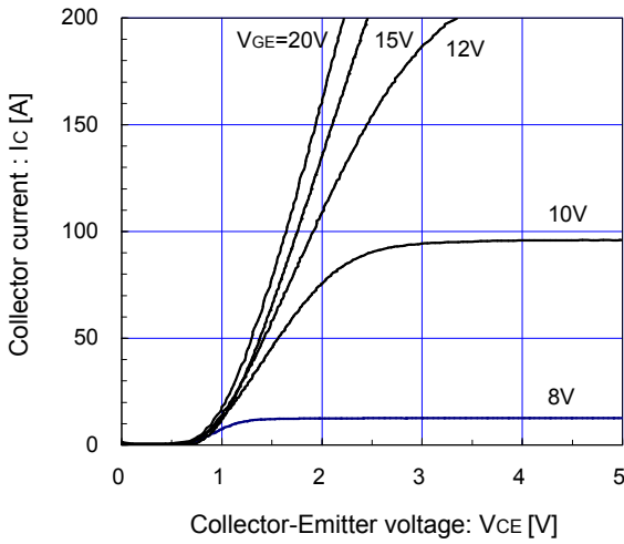
[ Inverter ] Collector current vs. Collector-Emittor voltage (typ.) T j = 25°C / chip
