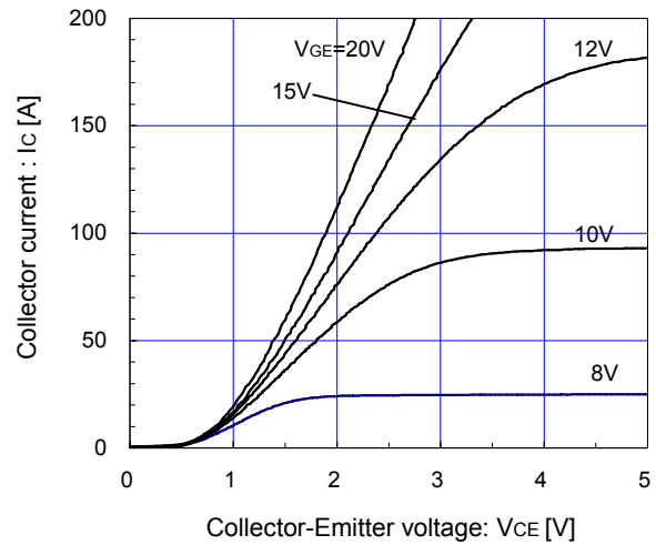
[ Inverter ] Collector current vs. Collector-Emittor voltage (typ.) T j = 150°C / chip
