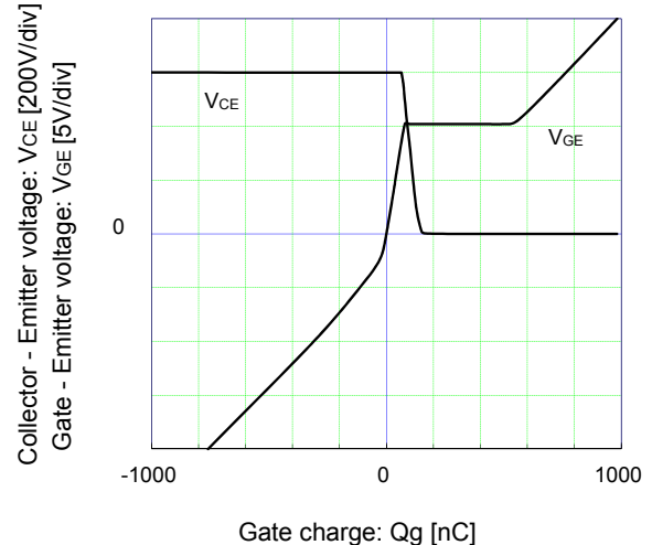
[ Inverter ] Dynamic gate charge (typ.) V CC =600V, I c =100A, T j = 25°C
