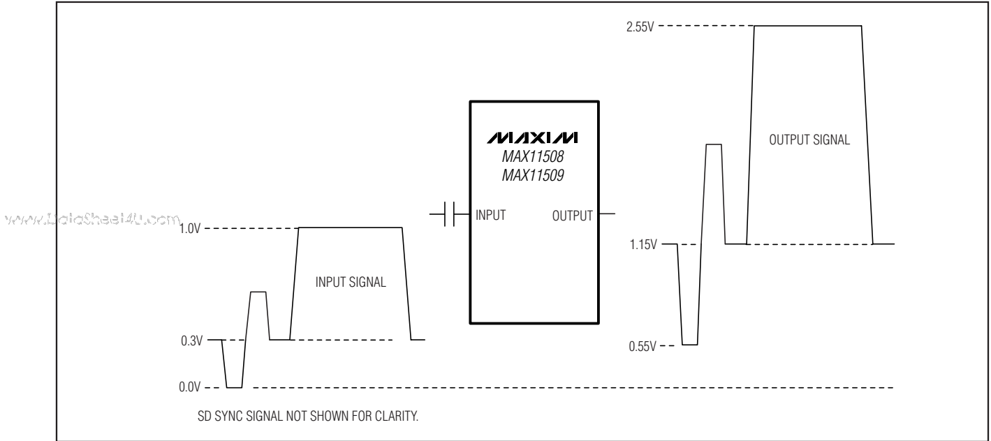
Figure 2. Typical AC-Coupled Signal
