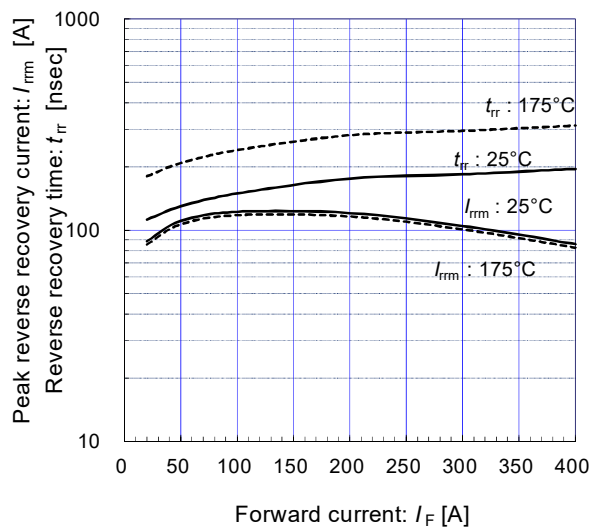
Reverse recovery characteristics (typ.) V_{CC} = 600\text{V} , V_{GE} = +15/-15\text{V} , R_G = 1.8\ \Omega
