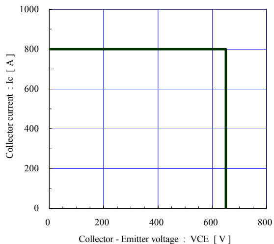
Reverse bias safe operating area (max.) +V_{GE}=15V, -V_{GE} \le 15V, R_g \ge 6.8\Omega, T_j \le 125^\circ C
